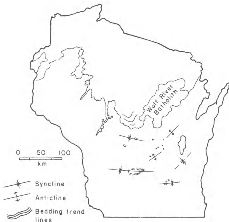
Figure 16. Major structures in the Baraboo interval rocks.
