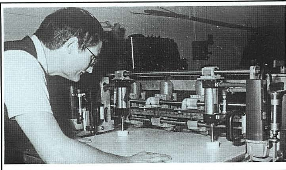
BISCUIT JOINTER PROTOTYPE - Dr. Tony Gillies from the Department of Civil Engineering is shown above with the automated prototype which he has developed with Dr. Murray Patterson to improve production for the Thunder Bay based company, Handcrafted-Cabinets.
